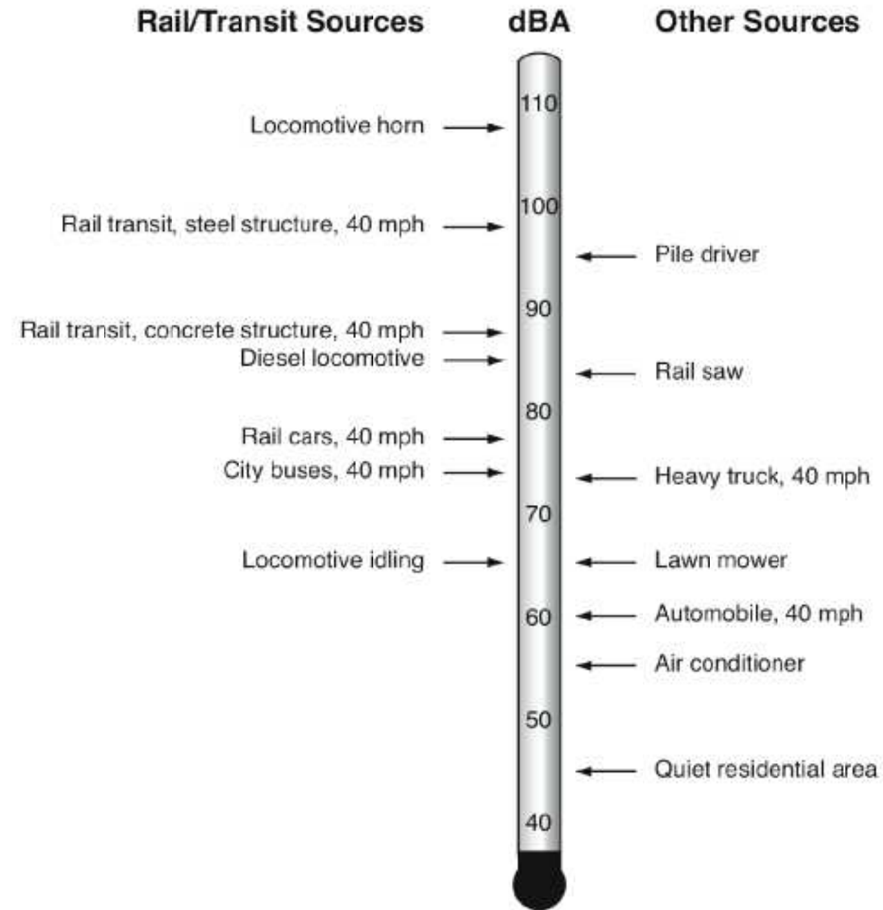
Typical A-weighted Sound Levels 100 ft. from Sources
